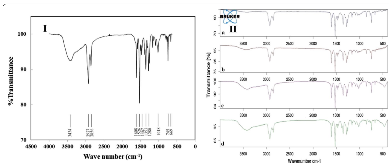
Fig. 4 FT-IR spectra of the fabricated \text{Fe}^{3+} selective membrane (I) and comparison of FT-IR spectra for membrane ingredients under different conditions (II): a newly dry fabricated membrane, b membrane saturated in iron solution for 24 h, c used membrane after 5 weeks and d used membrane after 15 weeks
