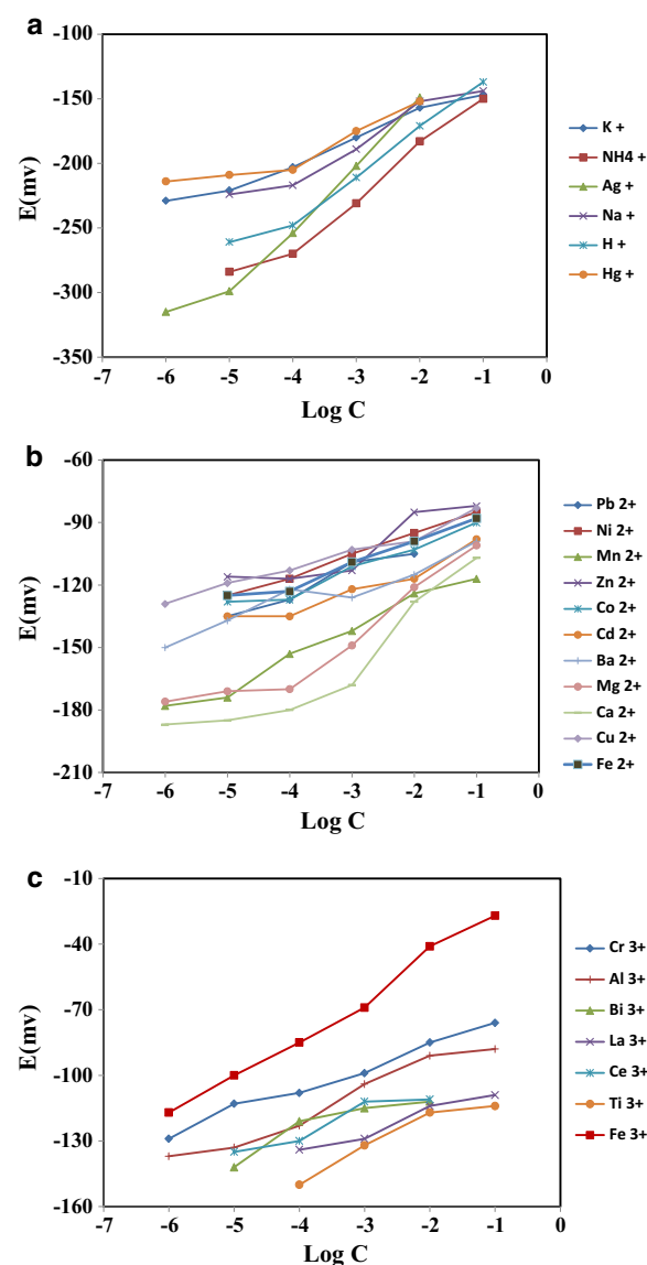
Fig. 2 The potential responses of PVC membrane sensor based on b-18C6 towards monovalent cations (a), bivalent cations (b), and trivalent cations (c) at 25 °C
