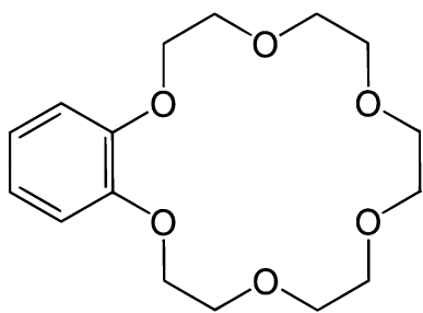
Fig. 1 Chemical structure of benzo-18-crown-6
